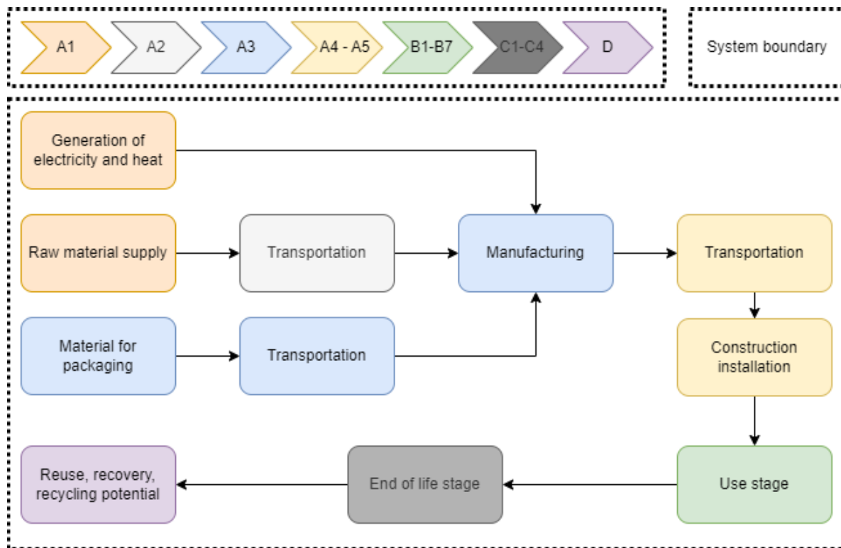
Figure 1 System boundary of the LCA study conducted on production of UKKO S
