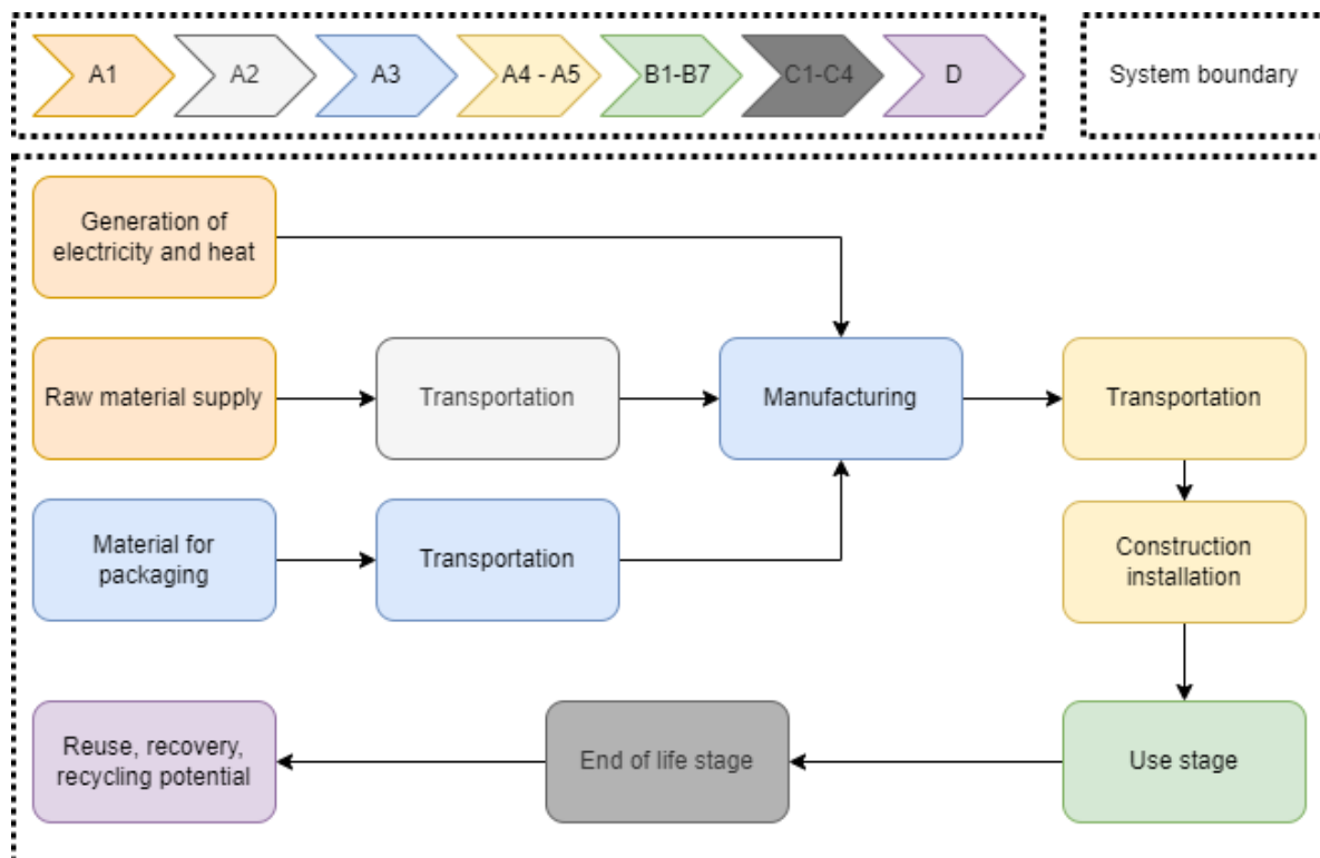
Figure 1 System boundary of the LCA study conducted on production of GEO FL S
