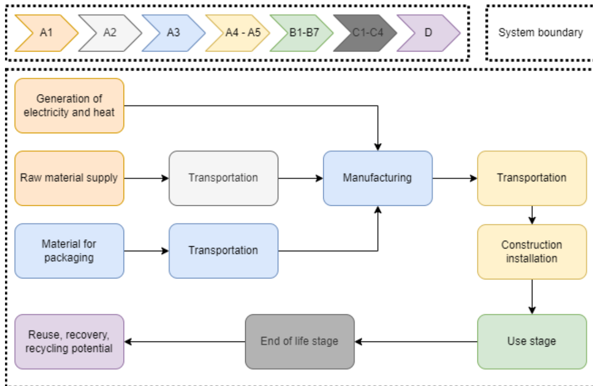
Figure 1 System boundary of the LCA study conducted on production of GEO ST M
